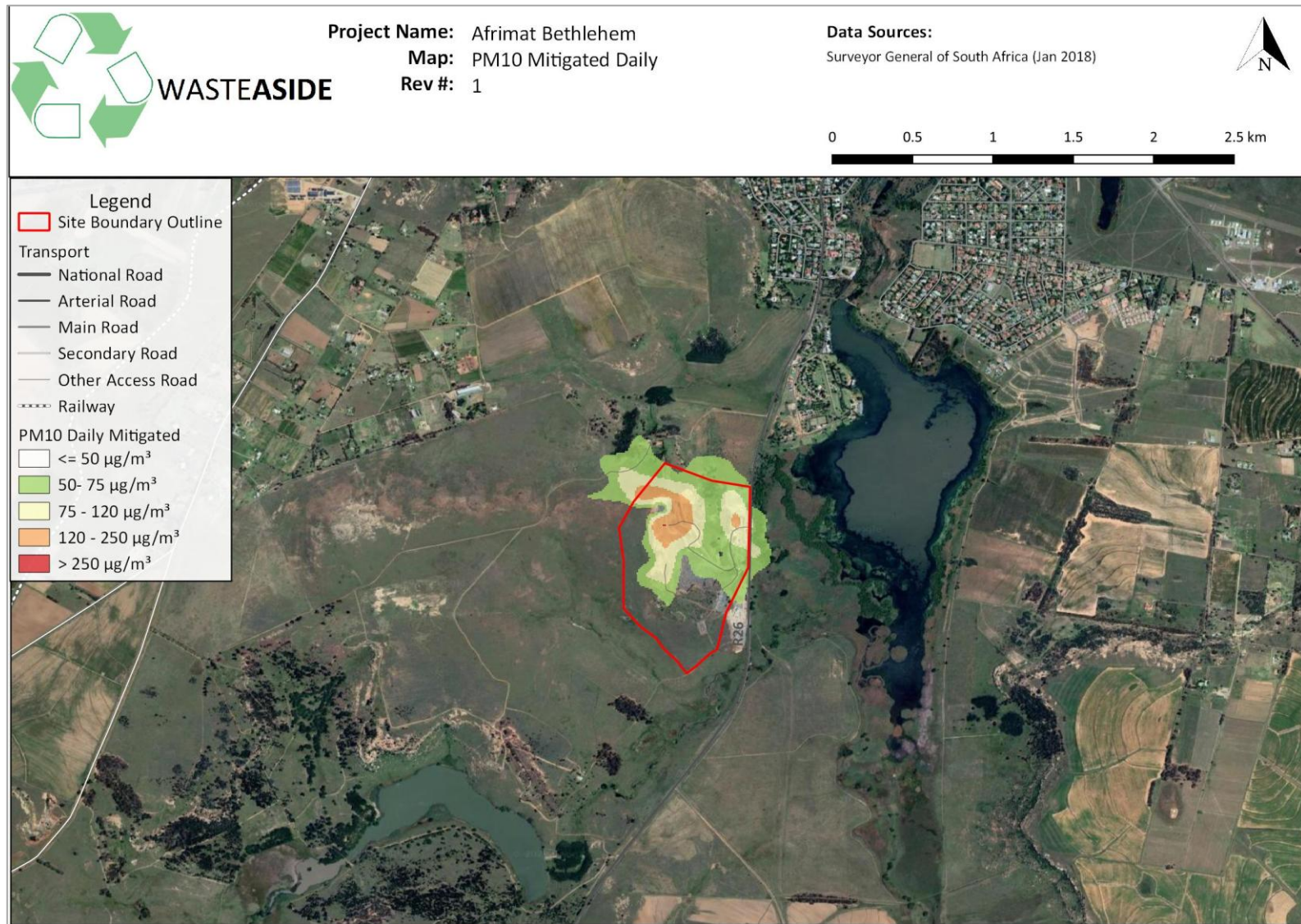
Figure 16: Predicted 2nd Highest daily concentrations for PM10 for the Afrimat Bethlehem project operations when mitigated
