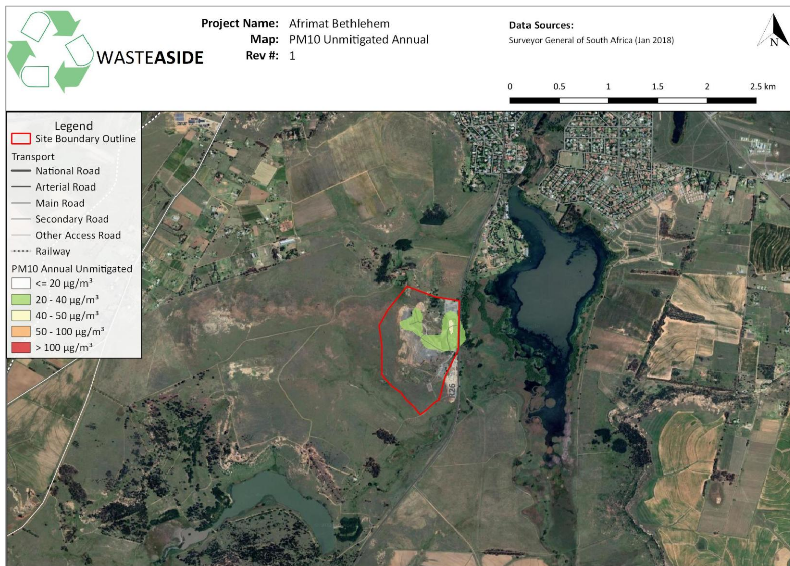
Figure 13: Predicted average annual concentrations for PM10 for the Afrimat Bethlehem project when unmitigated.
