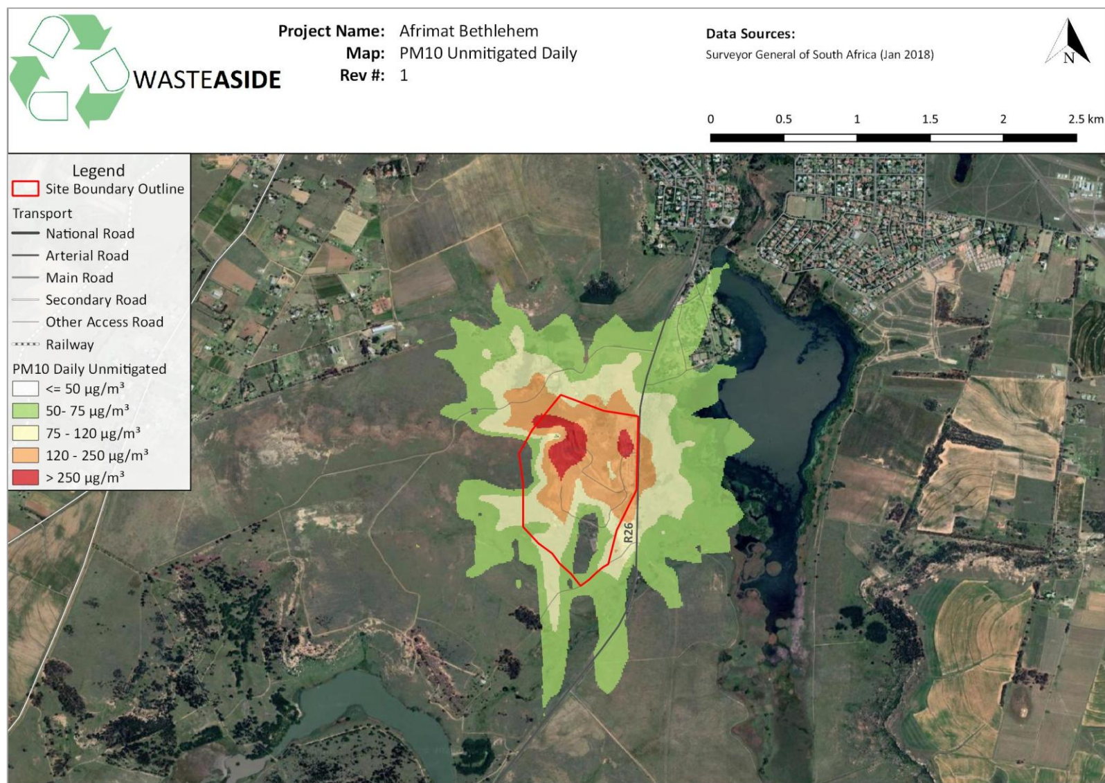
Figure 15: Predicted 2nd Highest daily concentrations for PM10 for the Afrimat Bethlehem project operations when unmitigated.
